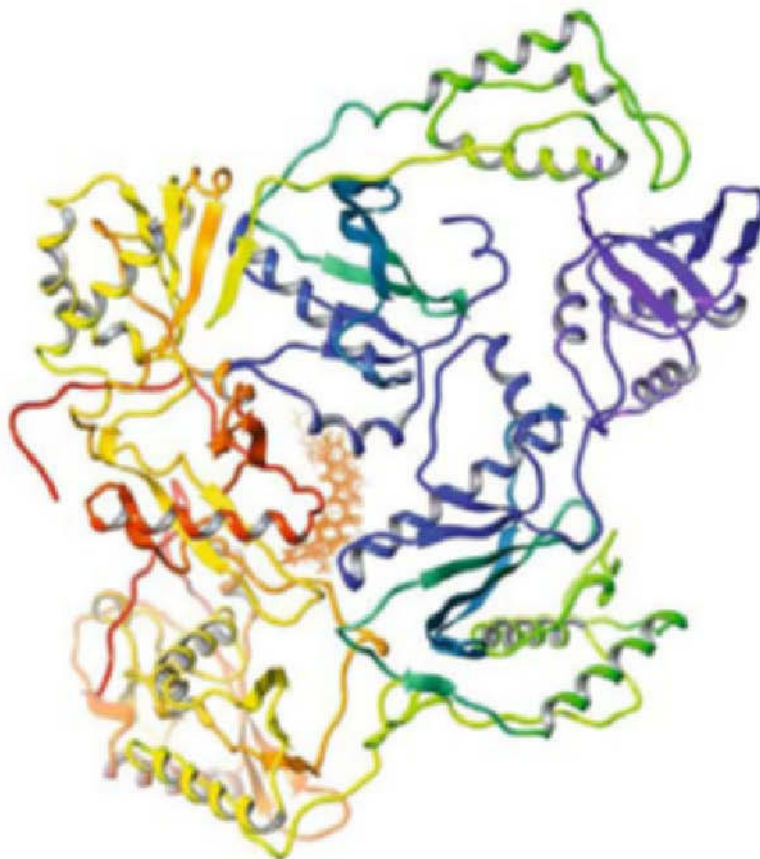
Figure 1. Binding of delvardine and its analogues into the p66 domain of HIV-1 RT.
