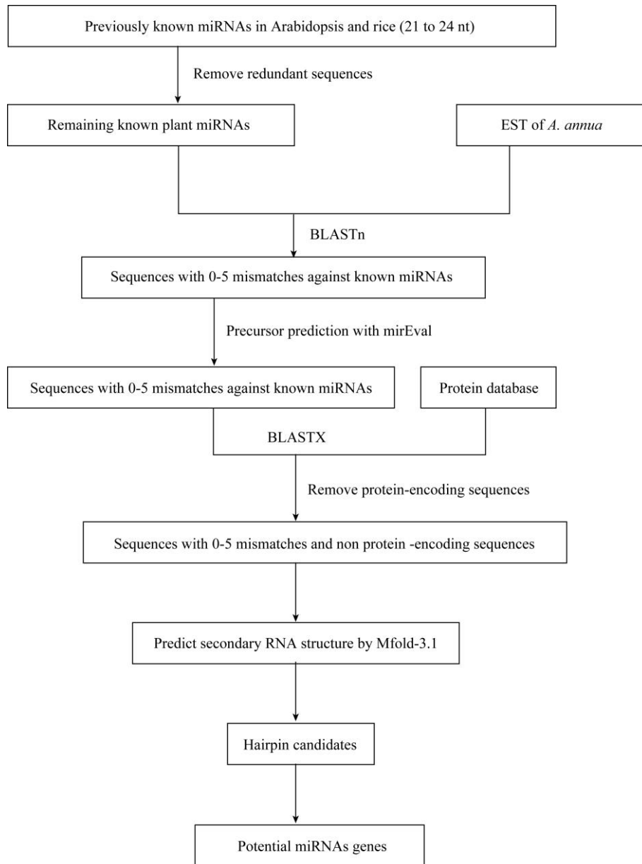
Figure 1 Schematic diagram for searching potential miRNA genes in A. annua by identifying homologs of previously known plant
