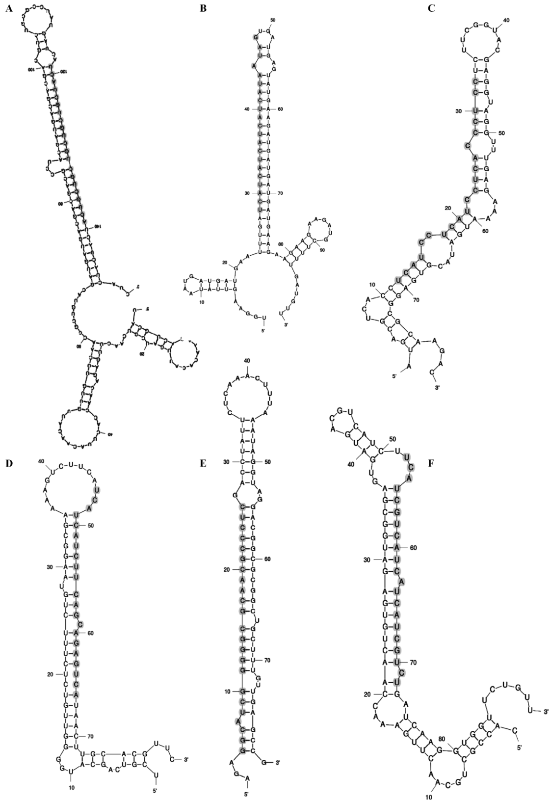
Figure 2 Mature and precursor sequences and the predicted stem and loop structures of newly identified miRNAs in A. annua . The mature miRNAs are highlighted in gray. A. miR-414 (EY064998; homolog of A. thaliana ); B. miR-414(EY057163; homolog of O. sativa ); C. miR-414 (EY082442; homolog of O. sativa ); D. miR-414 (EY107691; homolog of A. thaliana ); E. miR-1310 (EY057327;
