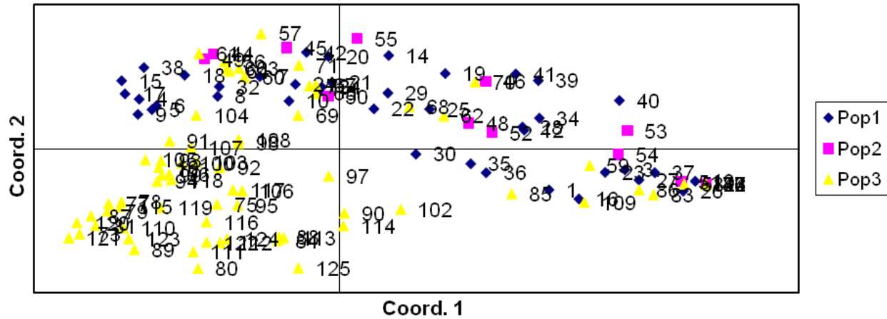
Figure 2. PCA analysis shows distribution of 3 groups as per their genetic relatedness.
