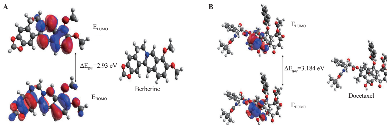
Figure 2. The higher occupied and lower unoccupied atomic orbitals (HOMO and LUMO) of (A) berberine and (B) docetaxel with an energy bandgap.
